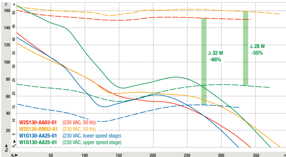
Fig. 2: Air performance measured in accordance with ISO 5801 installation category A
